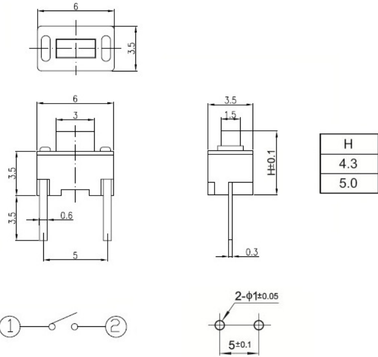
CIRCUIT DIAGRAM
